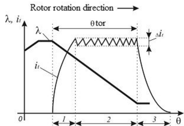
Fig. 2. Phase current in deceleration of BLDC motor
