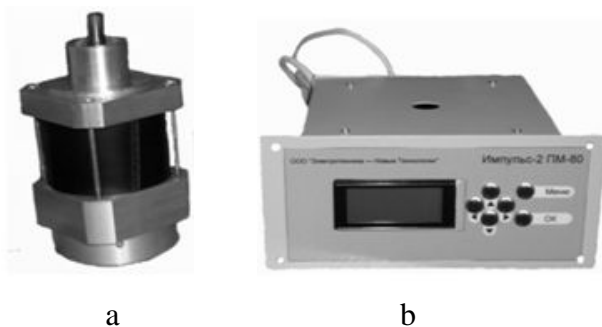
Fig. 4. BLDC drive for PEWF: a – BLDC motor; b – control unit
