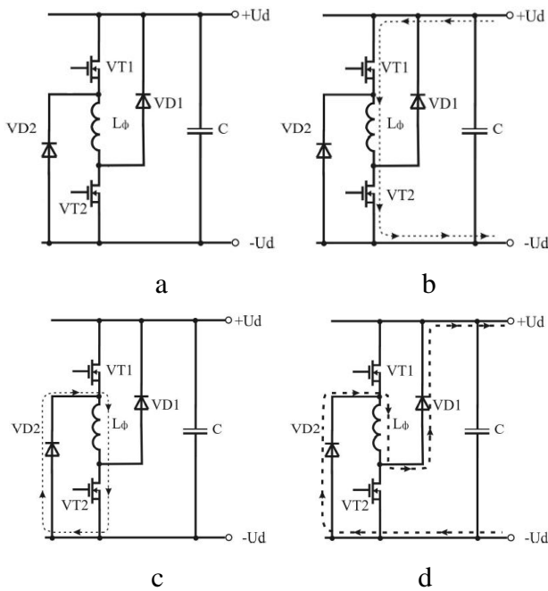
Fig. 3. Circuit of current control (a), and modes of operation of BLDC motor phase at two switched on transistors “P2” (b), one transistor “P1” (c), at both switched off “P0” (d)
