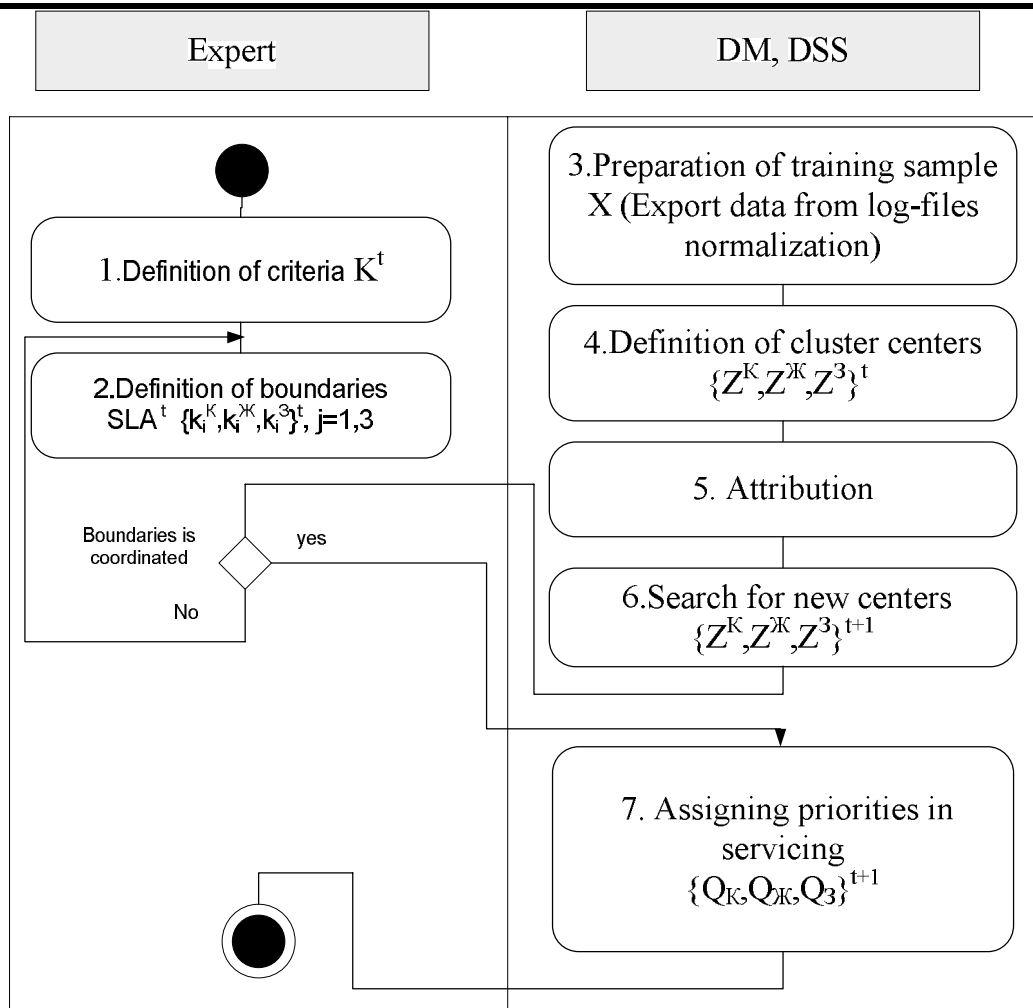
Fig. 1. Dynamic information technology, Classification Scheme of software applications
